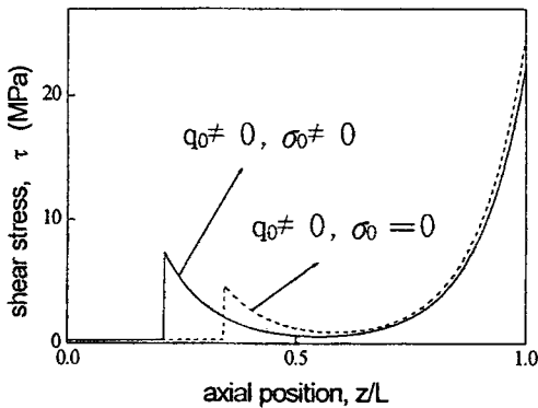
(b) Partially bonded
