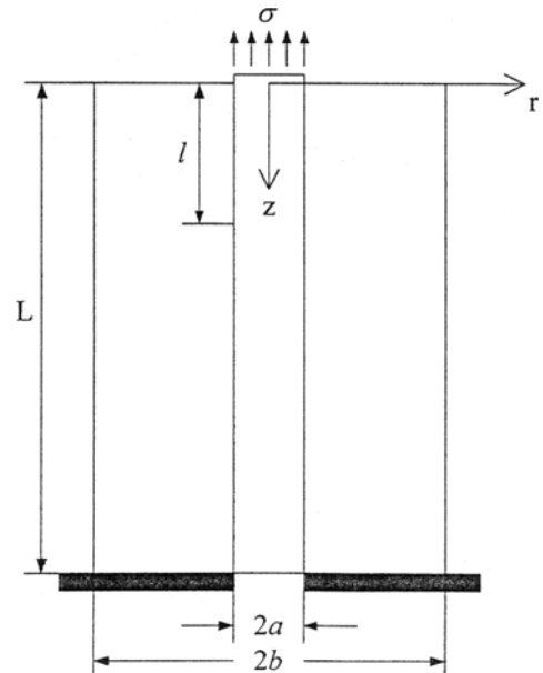
Fig. 1 Schematic of the single fiber pull-out model
